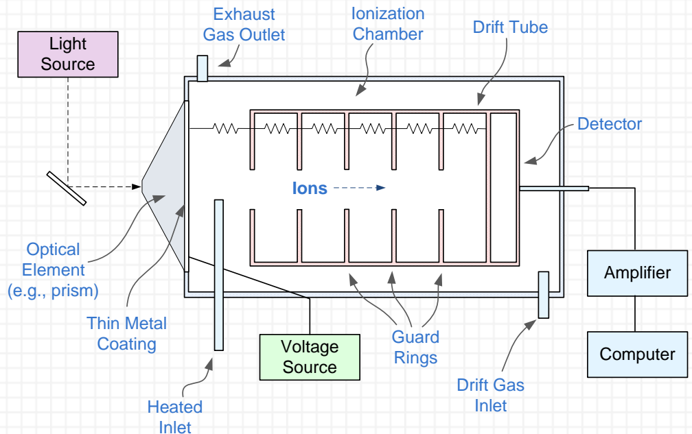
Figure 1: Schematic of Hazardous Chemical Detection Device
